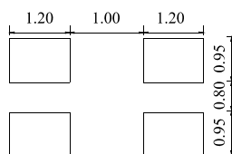
Recommended Solder Pattern
